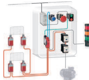
Safe stop 0 (PL d, SIL 2)
