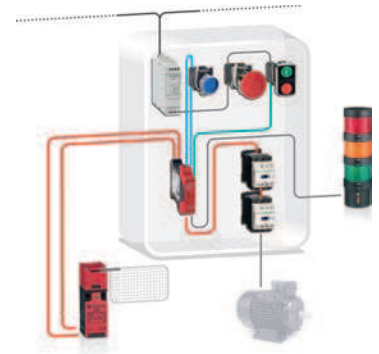
Safe stop 0 (PL e, SIL 3) High performance
