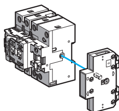
Early break and O and I signalling
