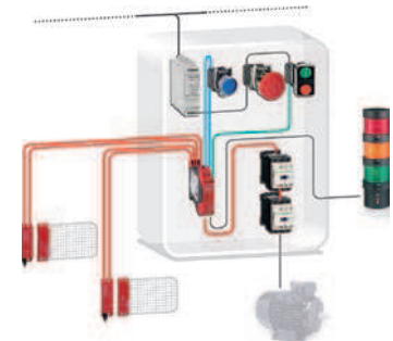
Magnetic switches (PL e, SIL 3)
